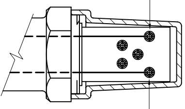
ENLARGED VIEW OF TEST POST HEAD
